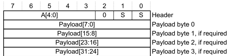
Figure D4-11 Instrumentation packet format
