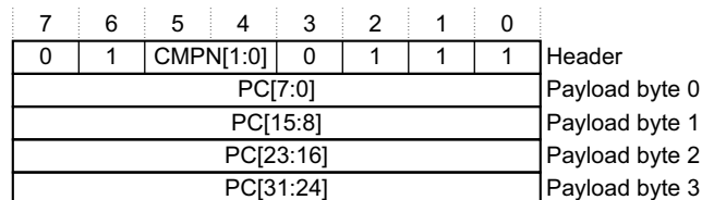
Figure D4-19 Data trace PC value packet format, IDs 8, 10, 12, or 14
